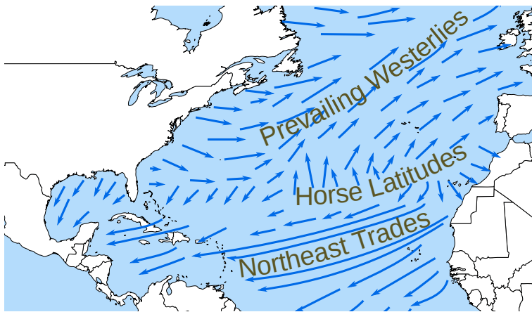
Figure 4.1: The Atlantic Trade Winds in January and July, adapted from Encyclopaedia Britannica.
